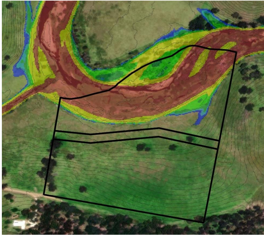
Figure 8: 1% AEP Flood Hazard Extract
