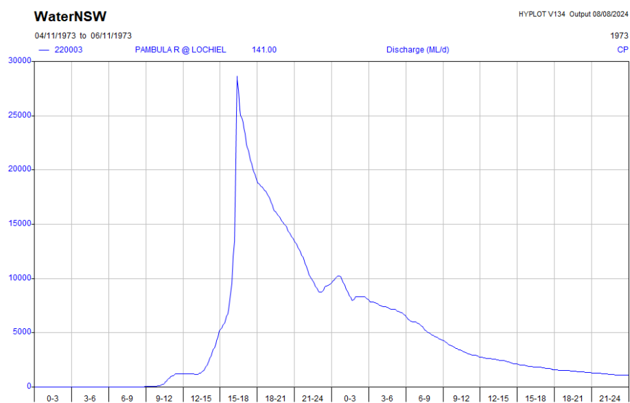
Figure 24: November 1973 Flood Hydrograph
