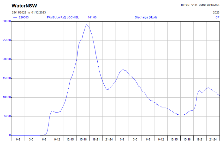
Figure 36: November 2023 Flood Hydrograph
