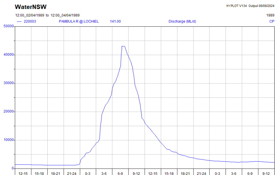
Figure 27: April 1989 Flood Hydrograph
