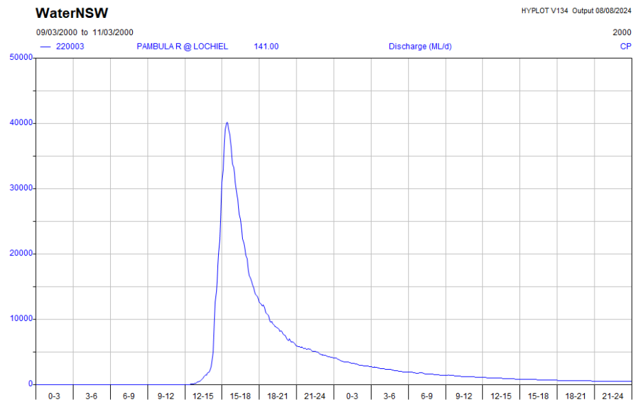
Figure 30: March 2000 Flood Hydrograph
