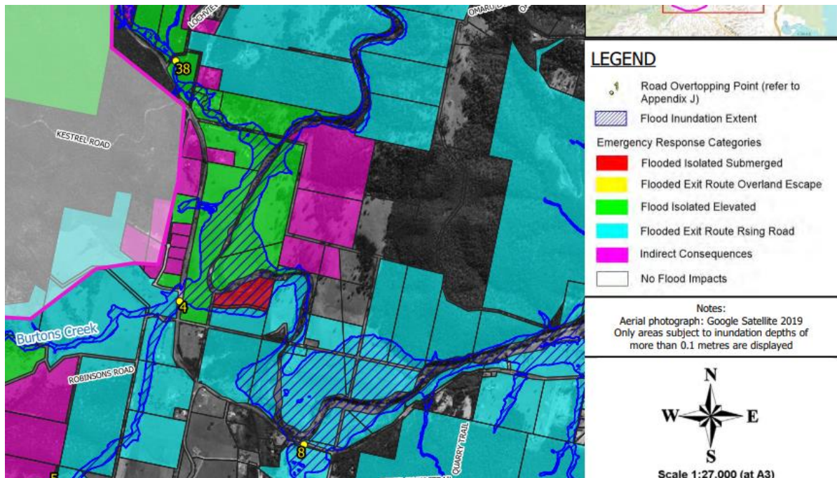
Figure 20: PMF FER Extract from Flood Study (Catchment Simulation Solutions, 2021, Figure 45.1)
