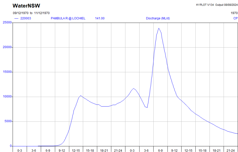
Figure 22: December 1970 Flood Hydrograph
