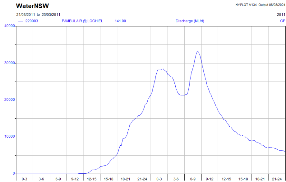
Figure 31: March 2011 Flood Hydrograph
