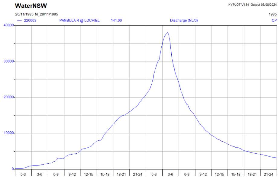
Figure 26: November 1985 Flood Hydrograph
