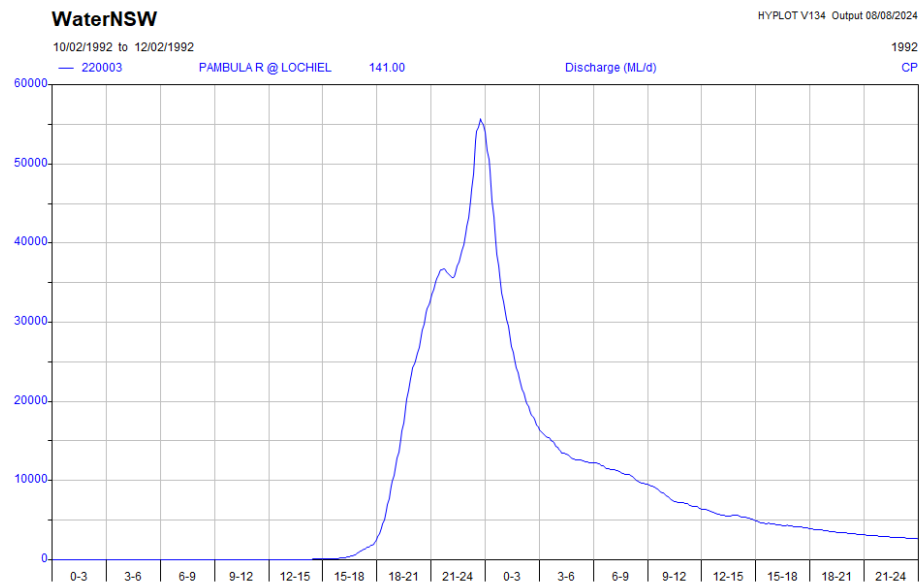
Figure 29: February 1992 Flood Hydrograph
