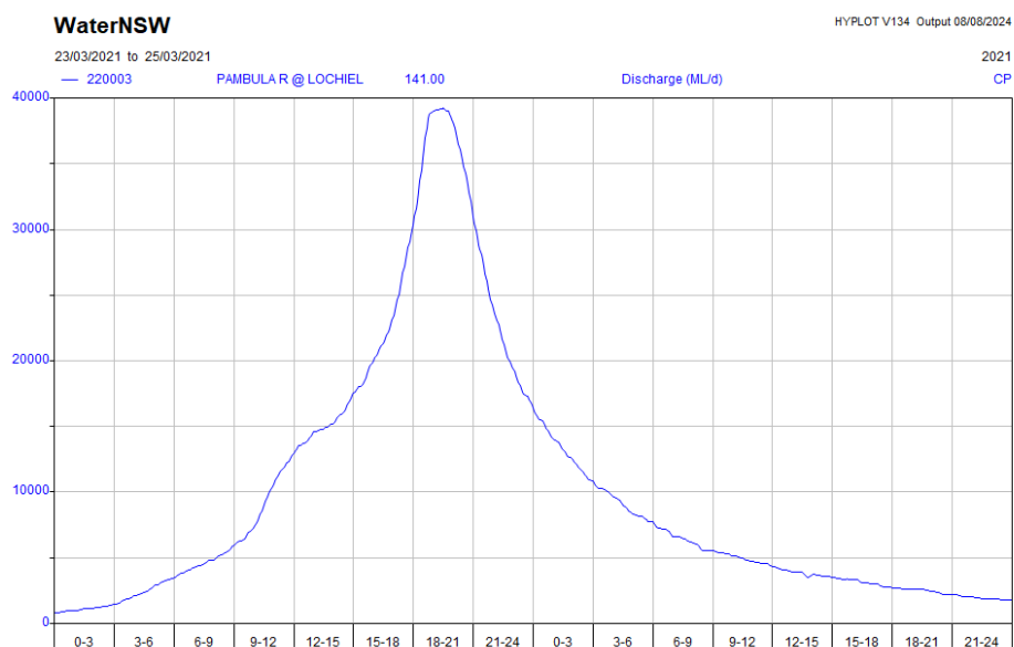
Figure 35: March 2021 Flood Hydrograph
