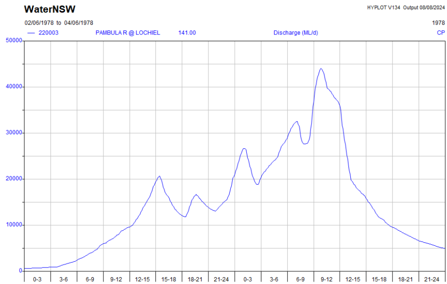
Figure 25: June 1978 Flood Hydrograph
